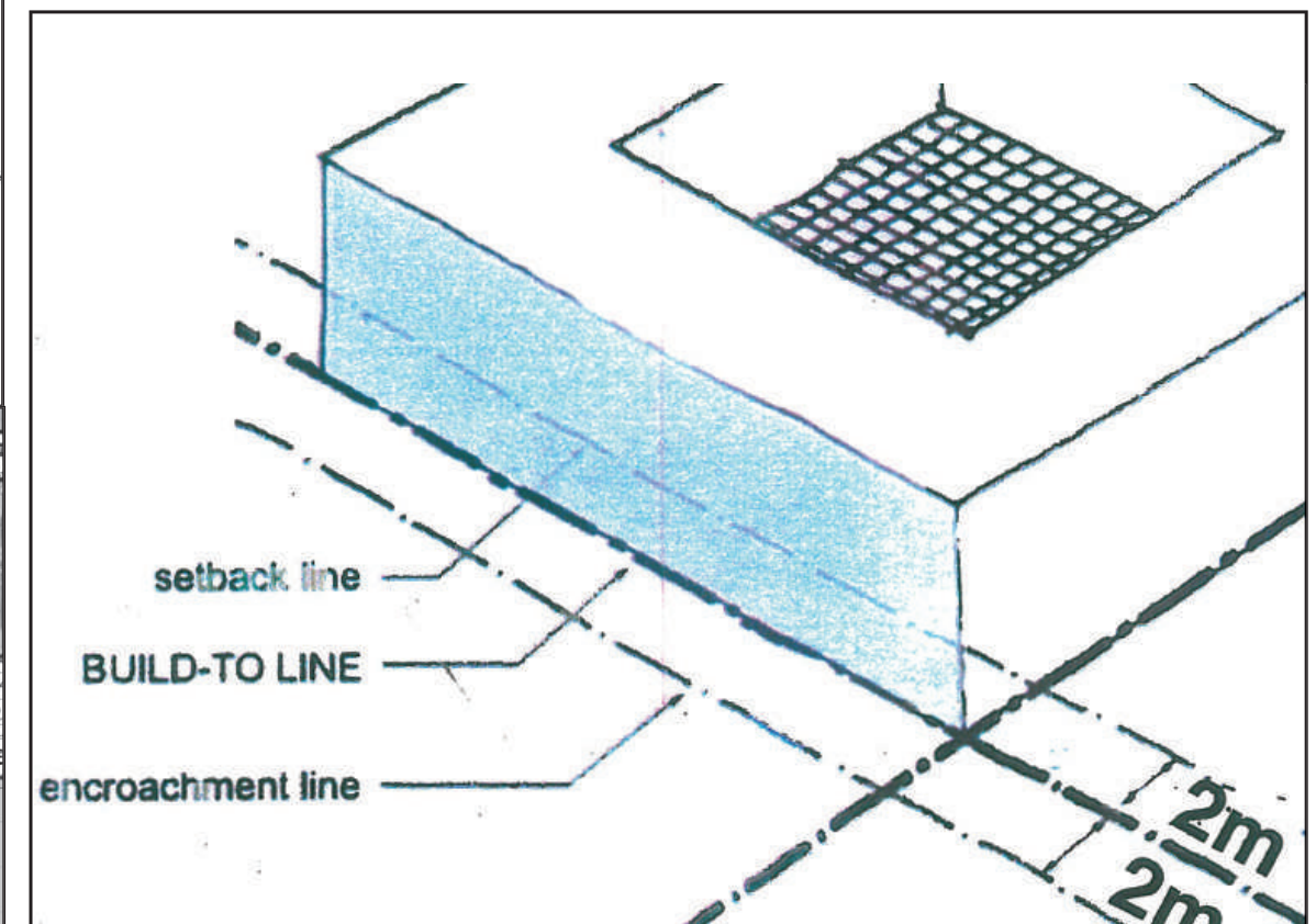
Fig 314:3 Concept sketches: Edge Definition_2003/08
