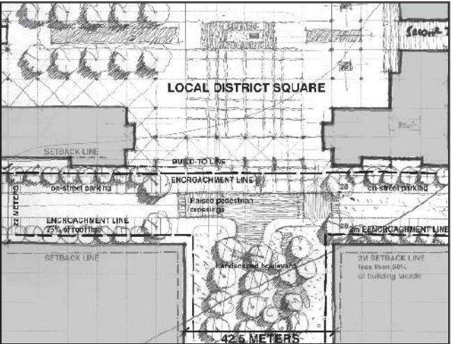
Fig23:3 EncroachmentandSet-back lines:Sketch3_2003/08
