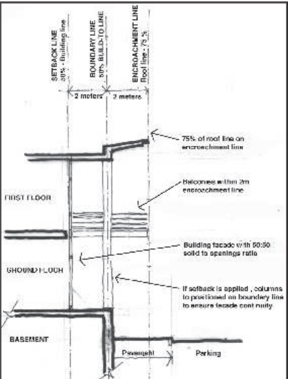
Fig21:3 EncroachmentandSet-back lines:Sketch3_2003/08
