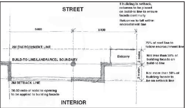
Fig22:3 EncroachmentandSet-back lines:Sketch2_2003/08
