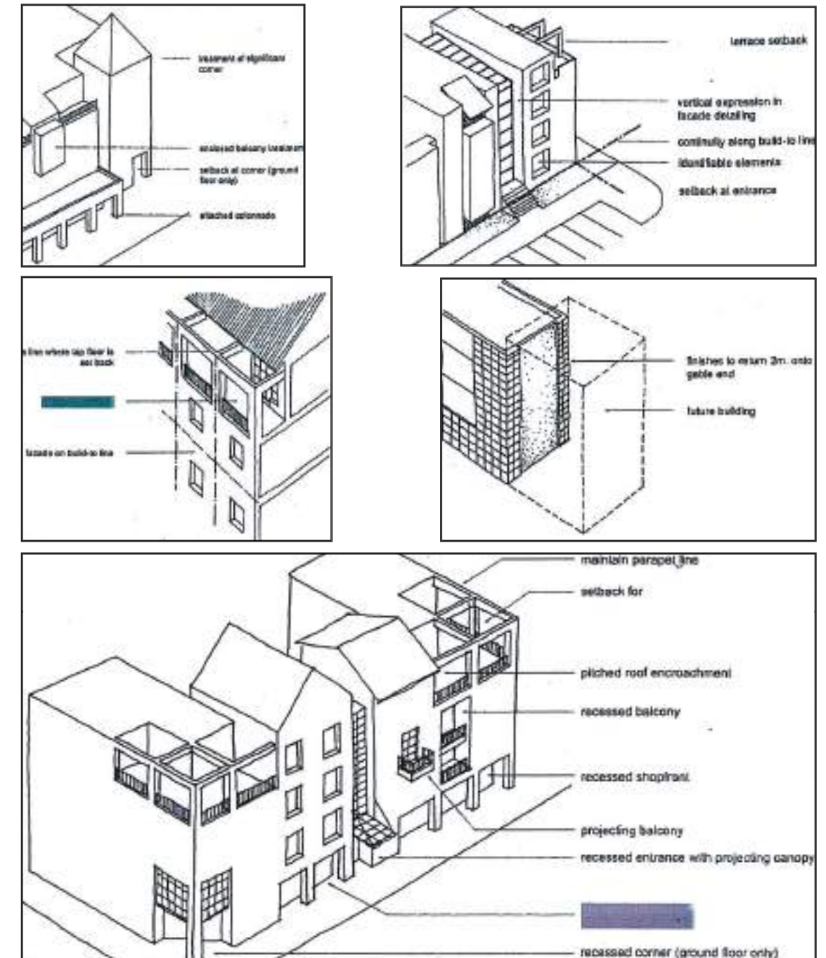
Fig 43: Diagrammatic representation of elevation elements_2008/03
