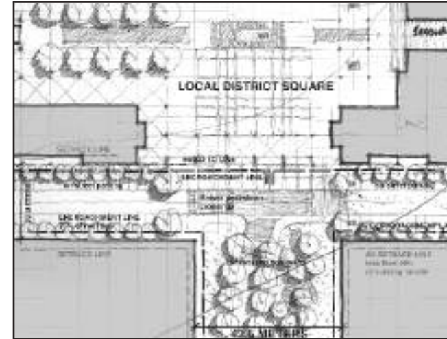
Fig 23: Encroachment and set-back lines: sketch 3_2003/08
