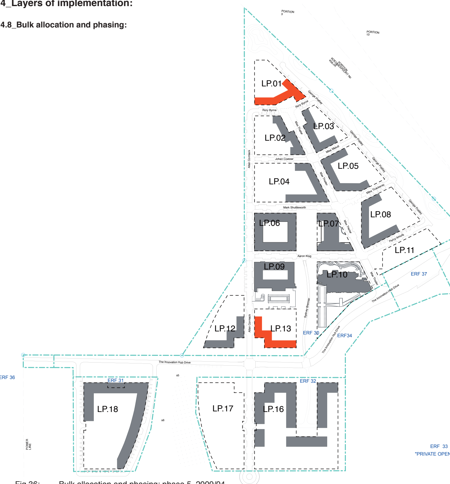
Fig 36: Bulk allocation and phasing: phase 5_2009/04
