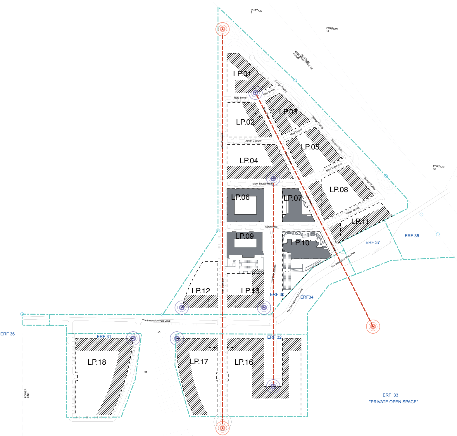
Fig 15: Edge Definition and legibility_2009/03
