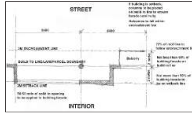
Fig 22: Encroachment and set-back lines: sketch 2_2003/08
