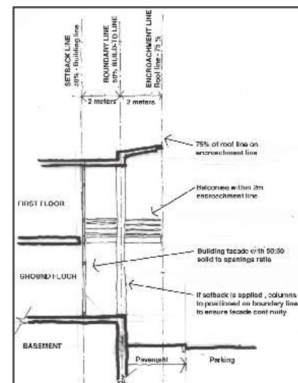
Fig 21: Encroachment and set-back lines: sketch 1_2003/08
